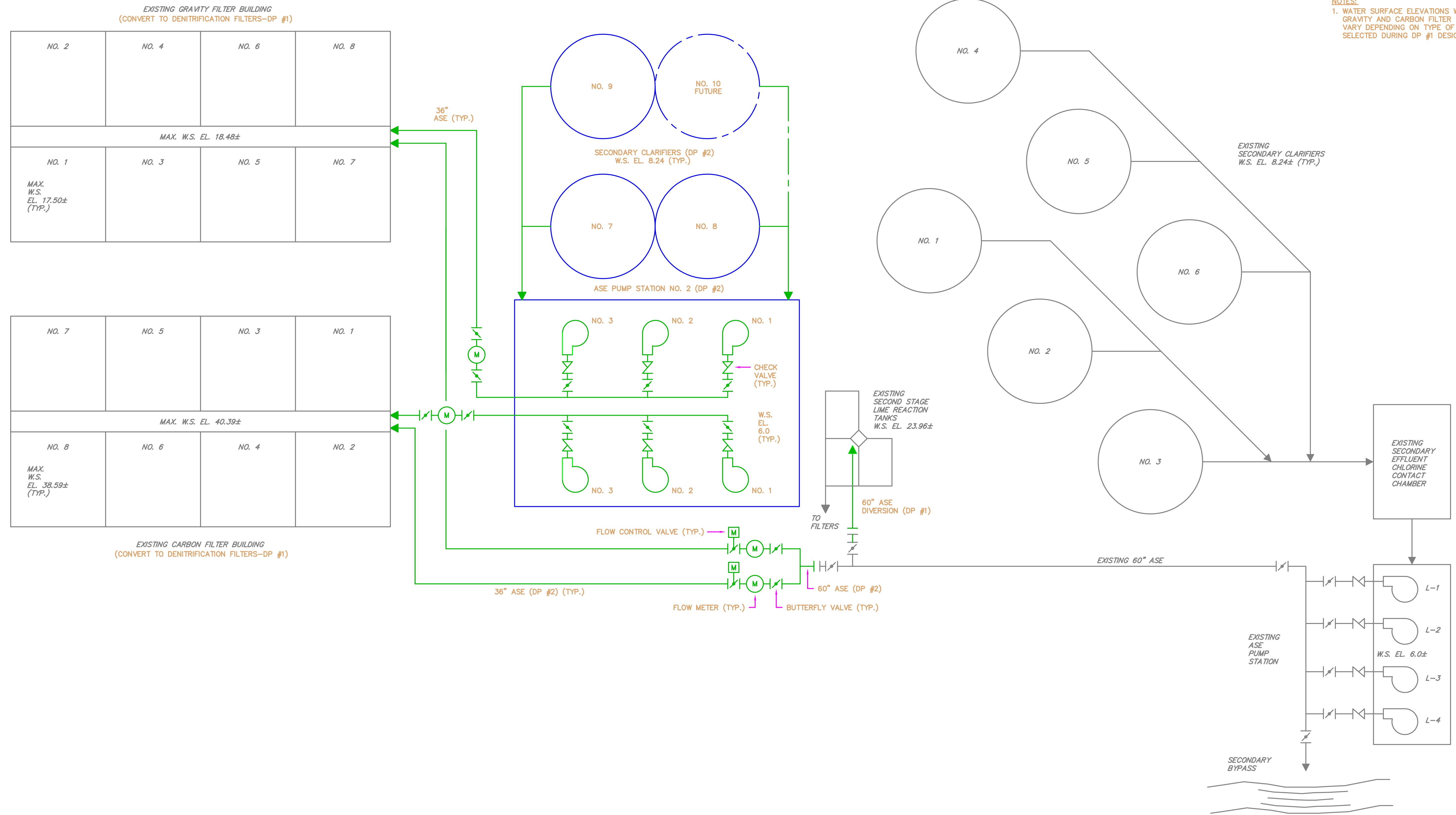
PROCESS FLOW DIAGRAM NOT TO SCALE
